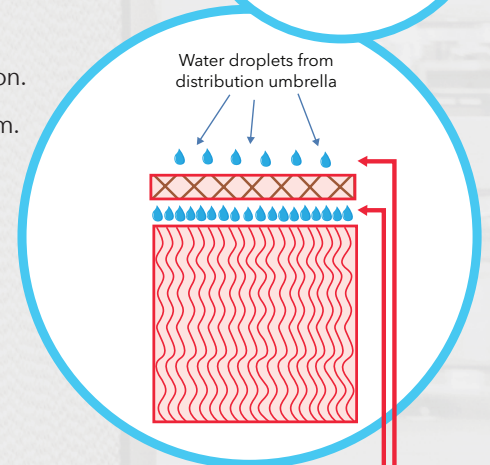
Water distribution media expands water distribution evenly.
